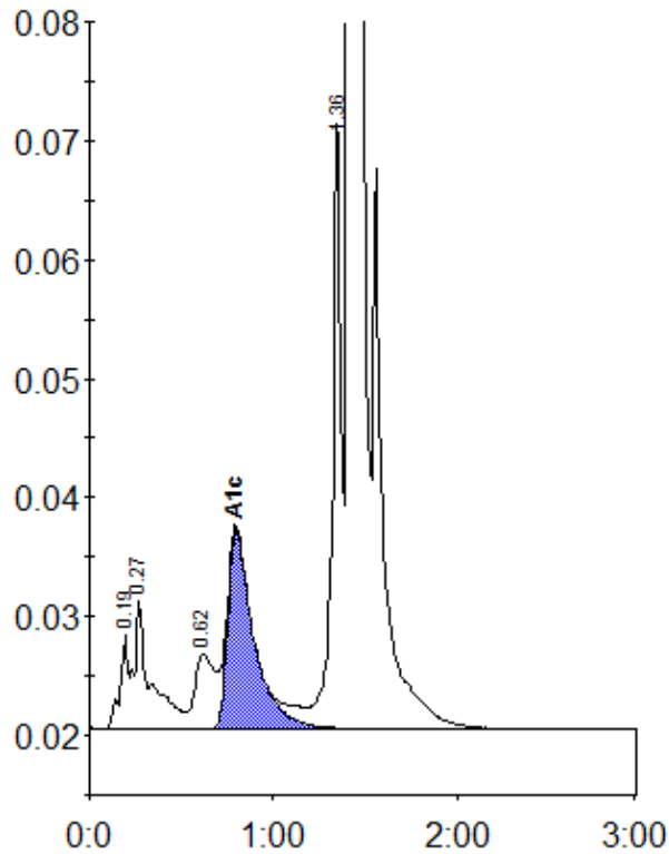
Peak table - ID: 10500144
